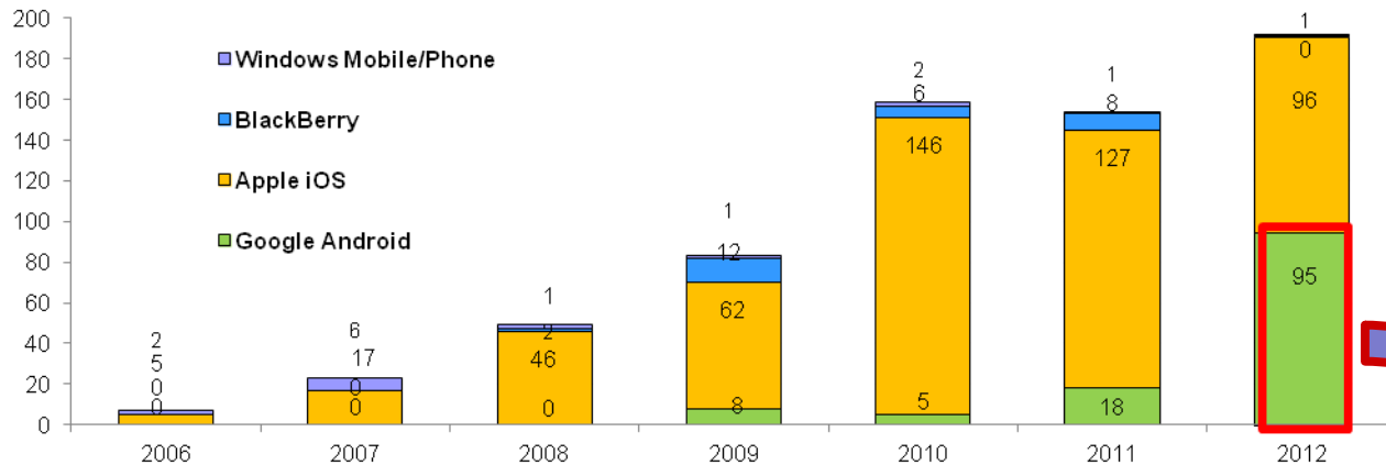
Vulnerabilities in Smartphone Applications by OS Platform
