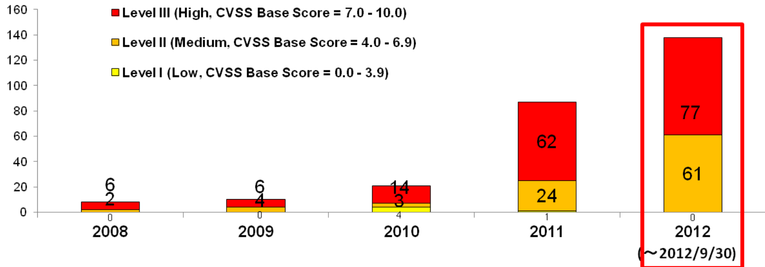
Number and Severity of Vulnerabilities in Industrial Control System Software
