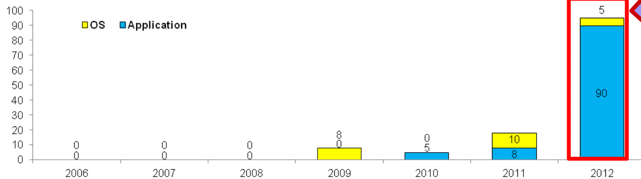
Number of Vulnerabilities in Android OS Software by Software Type
